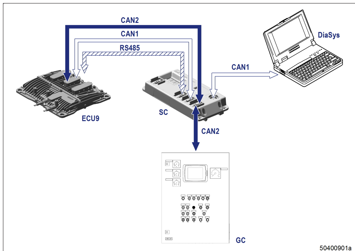
Figure 1: System overview – Example of a system featuring SmartConnect
